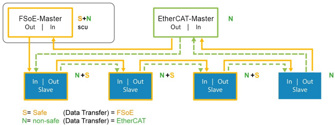
Fig. 3: Example FSoE network; safe and standard /non-safe data transfer
