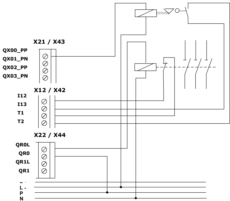
Fig. 30: Dual-channel output with relay output and semi-conductor output – external control circuit with monitoring
