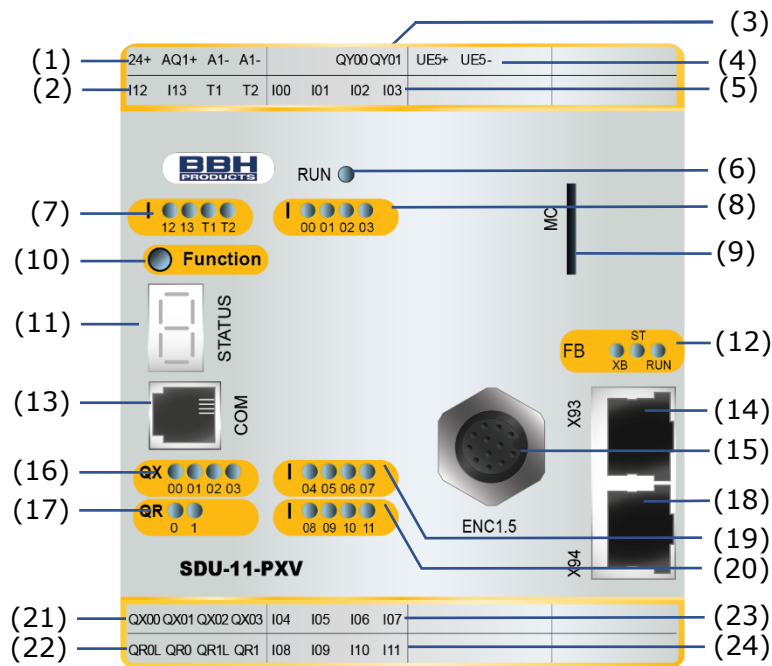
Fig. 6: structure of SDU-11-PXV
