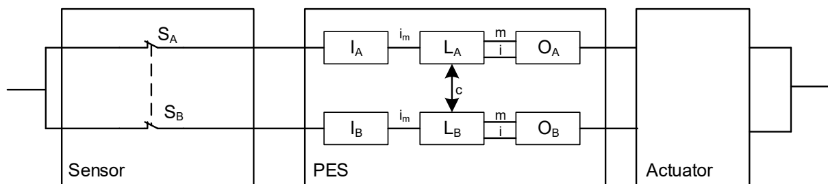
Fig. 13: Digital sensor 2-channel parallel
