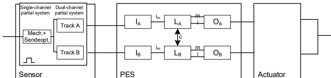
Fig. 22: Sensor system with single-/dual-channel partial system
