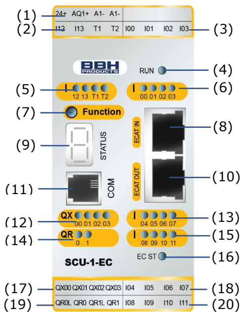
Fig 4: structure of SCU-1-EC
