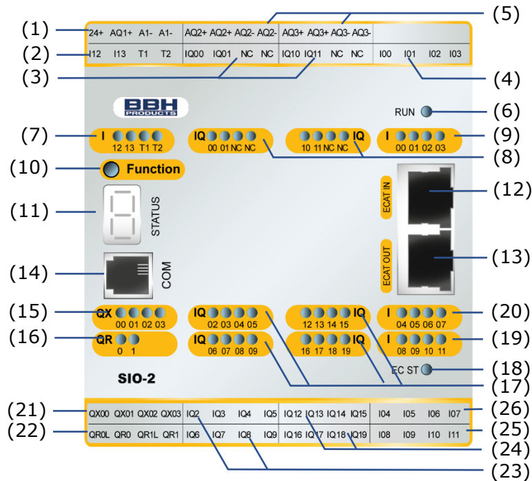
Fig. 8: structure of SIO-2
