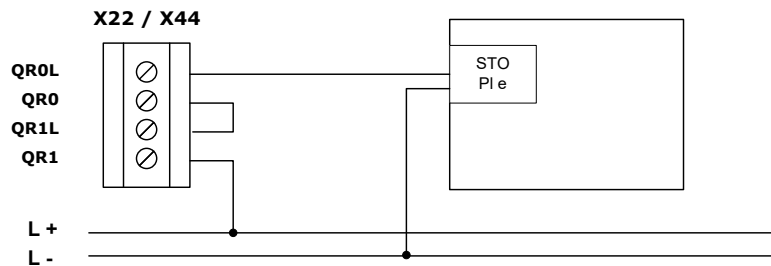
Fig. 31: Dual-channel output with relay output – external control circuit in PL e
