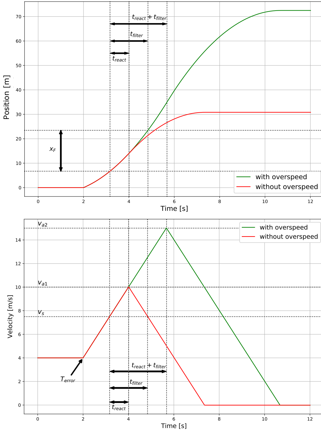
Diagramm 1: Drive response with / without overspeed distance
