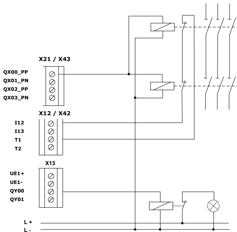
Fig 27: Single-channel switching output QX00_PP with dual-channel external circuit and monitoring at output 13 as group feedback
