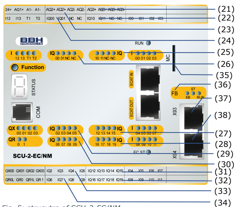
Fig. 5: structure of SCU-2-EC/NM
