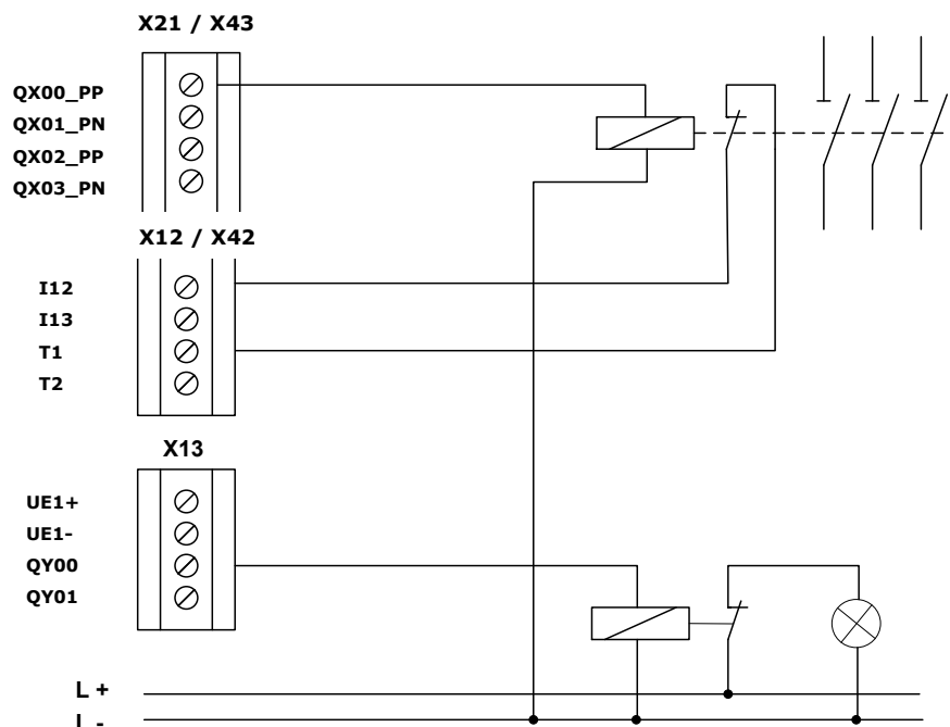
Fig. 26: Single-channel relay output with testing
