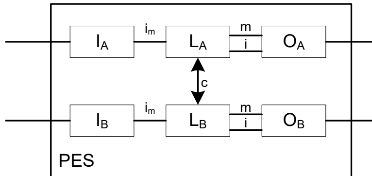
Fig. 11: 2-channel architecture
