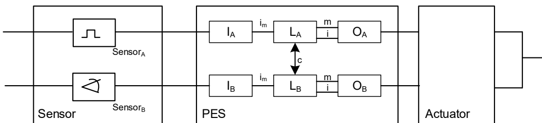
Fig. 21: dual-channel sensor system with separate signal processing
