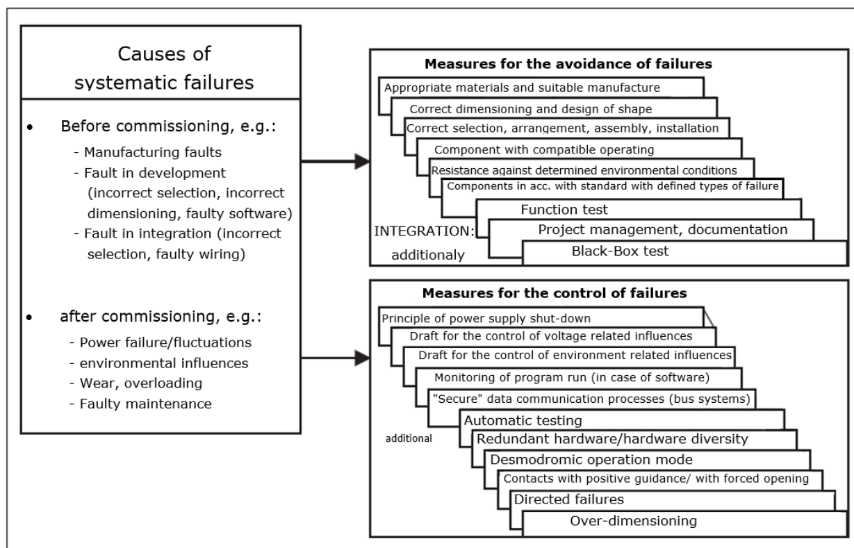
Fig. 67: Systematic failures
