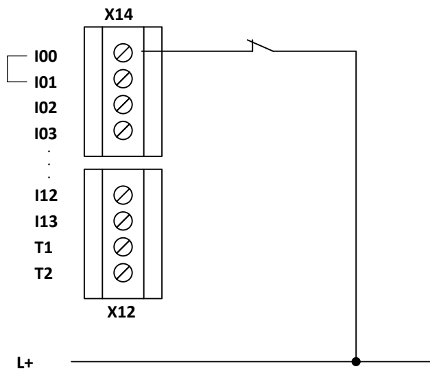
Fig. 16: Single-Channel sensor, without cross-shorting test
